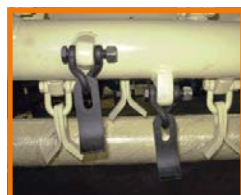
Slice knives for herbs and shrubs max Ø 3 cm. ROTOR I
